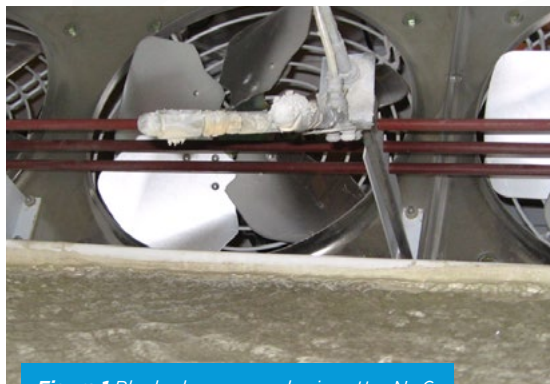
Figure 1 Blocked spray nozzles in setter No.6
