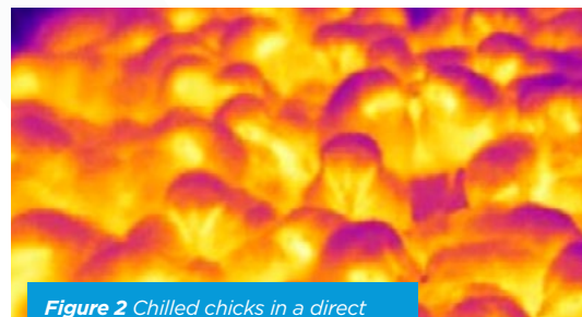
Figure 2 Chilled chicks in a direct draught from a ceiling air inlet.
