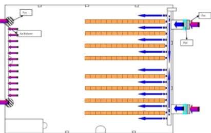
Figure 1 A typical laminar flow ventilation system for a chick holding room.
