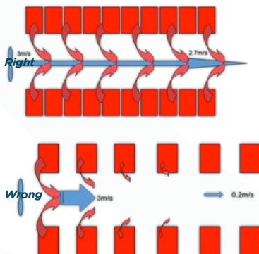
Figure 1 Comparison of chick box layout and resulting air speeds in properly and incorrectly laid out rooms.
