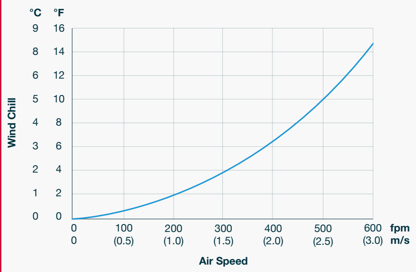
Figure 6.21 Theoretical cooling effect felt by a 3.5 kg (7.7 lb) broiler at an air temperature of 29.4°C (85°F).
