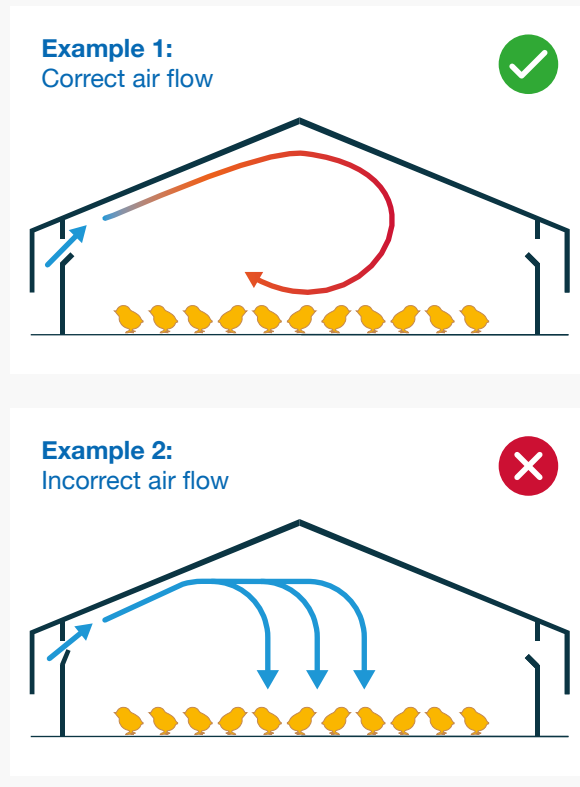
Figure 6.14 Illustration of air flow into the house. The picture on the top shows a correct air flow during minimum ventilation. The picture on the bottom shows an incorrect air flow during minimum ventilation.
