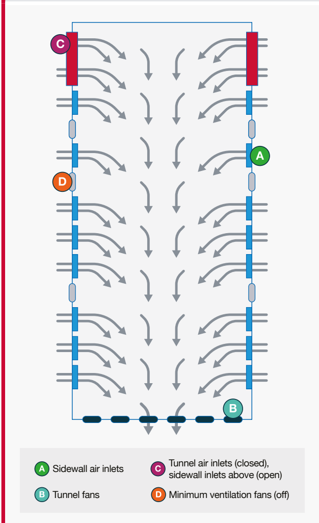
Figure 6.16 Typical air movement during transitional ventilation.
