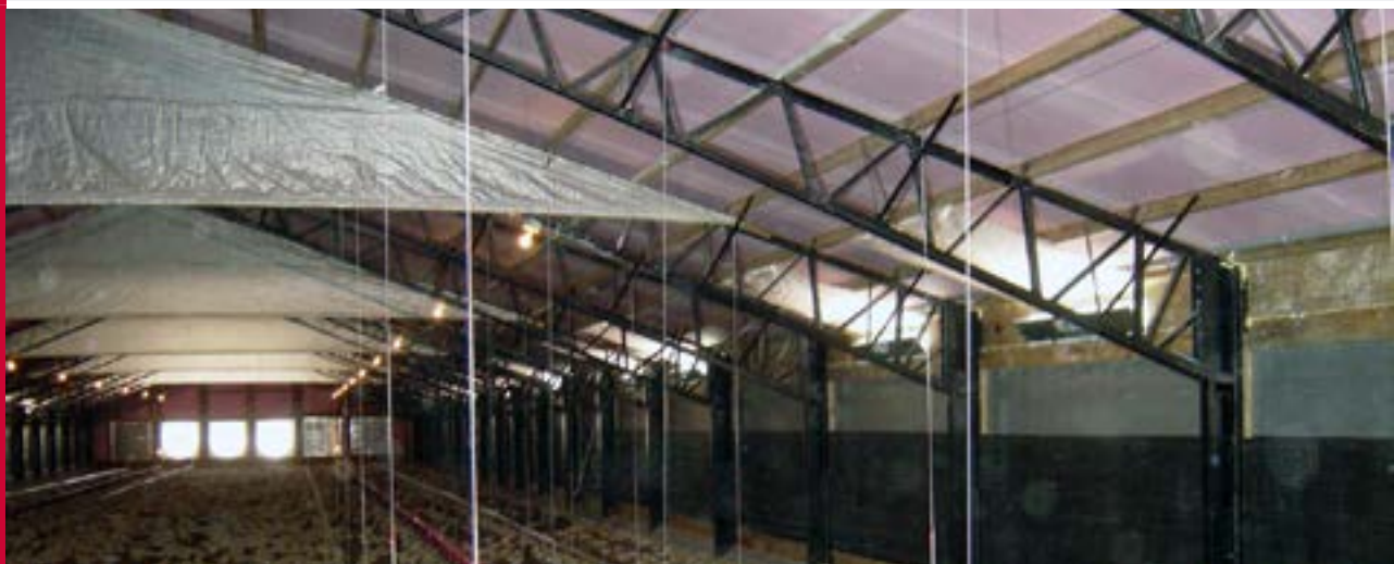
Figure 6.19 Example of air deflector/baffle placement in a tunnel-ventilated house.
